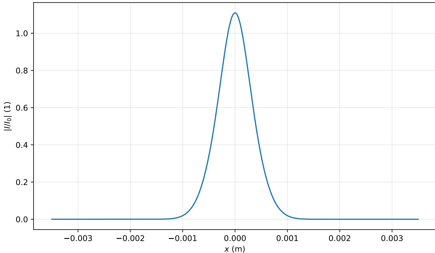
Intensity profile I(x, y = 0, z = 0.478m)/I_0 , P_{in}=0.8P_{cr} , artificial time
